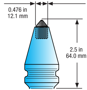
DR35 Carbide Plug
