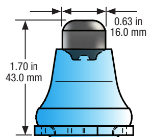
GWX28 Valve-Seat Carbide Tip
